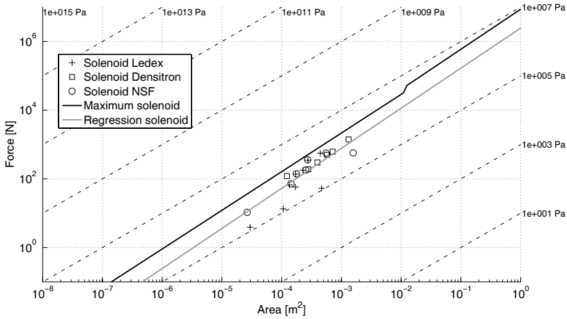
Fig. 3.19 Industrial electromagnetic actuator force-area comparison
