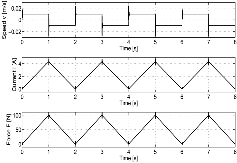
Fig. 4.16 Speed, current and force of the moving coil actuator tracking a triangular reference
