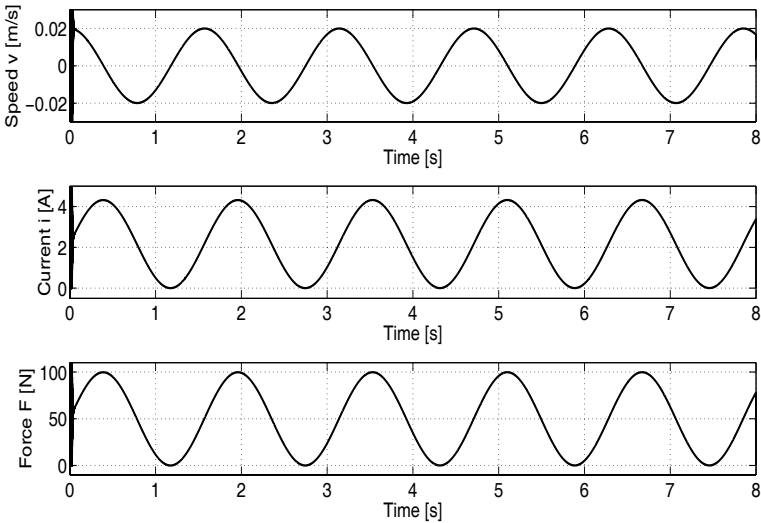
Fig. 4.18 Speed, current and force of the moving coil actuator tracking a sinusoidal reference
