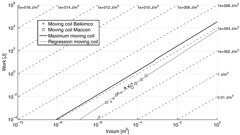
Fig. 4.11 Industrial electromagnetic actuator work-volum comparison
