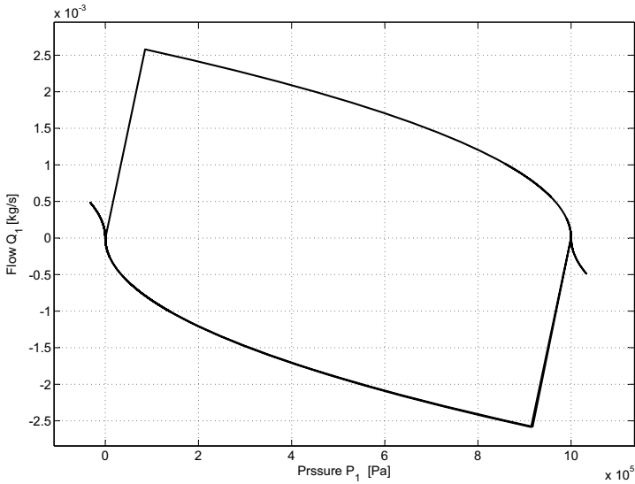
Fig. 5.17 Pressure-flow curve response of the hydraulic actuator to an open loop simulation. Simulation 2
