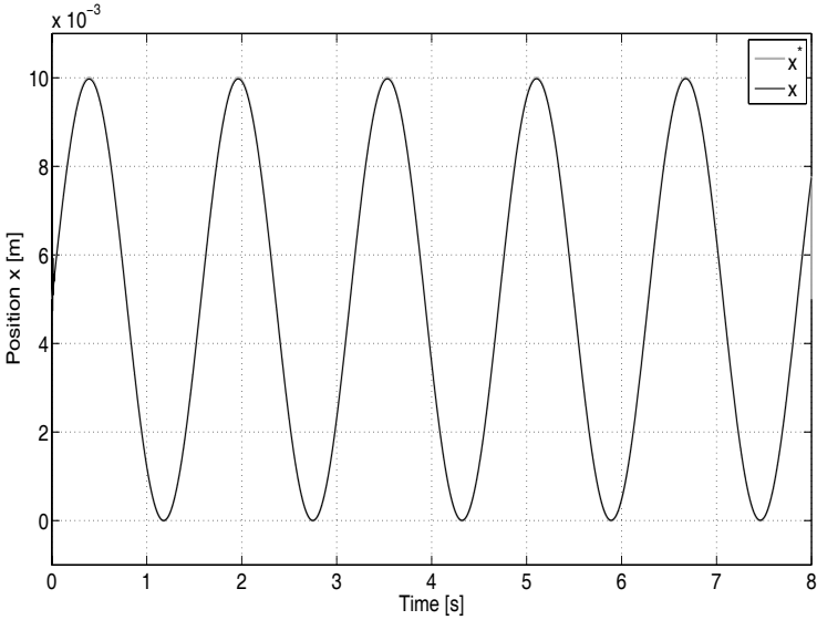
Fig. 4.17 Moving coil actuator response tracking a sinusoidal reference
