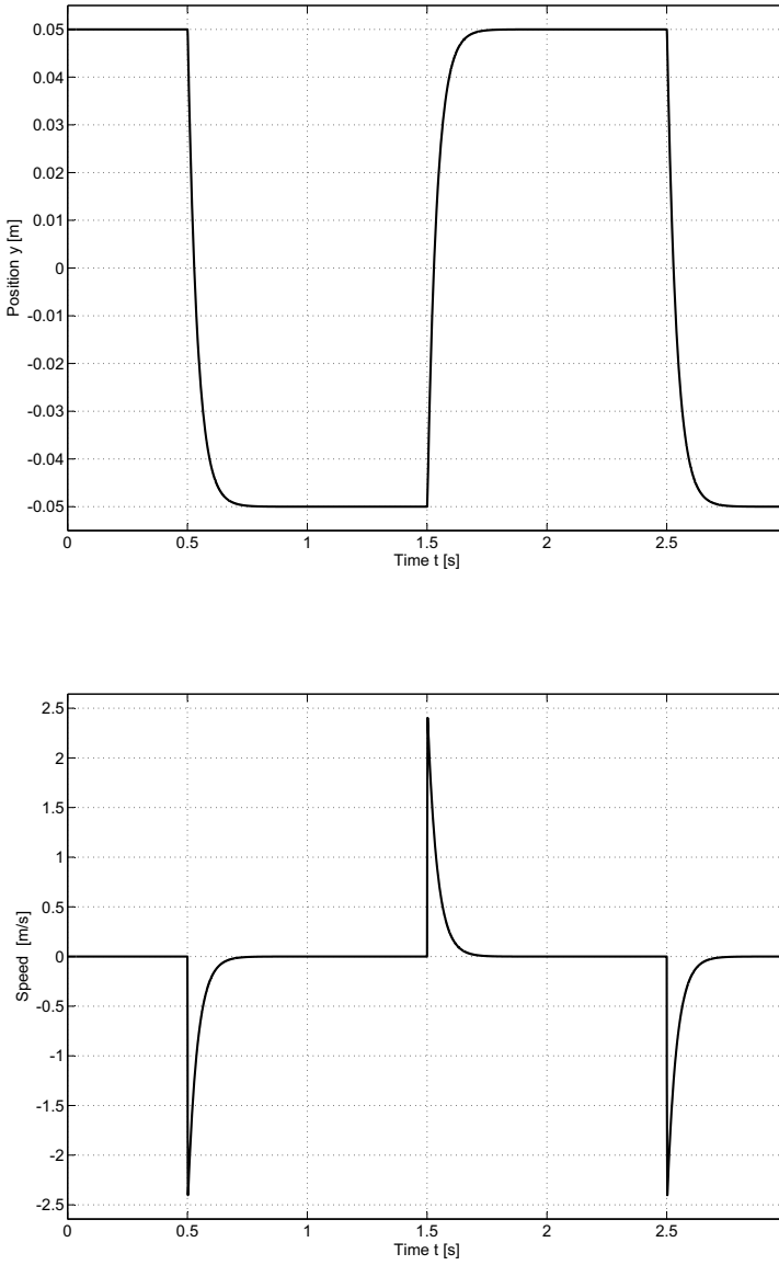
Fig. 5.10 Position and speed response of the hydraulic actuator to an open loop simulation. Simulation 1
