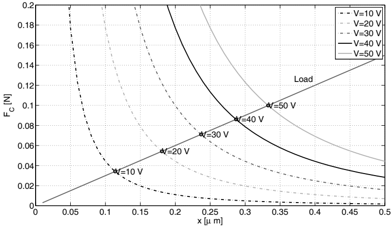
Fig. 2.19 Force-stroke curve equilibrium points of Example 2.5
