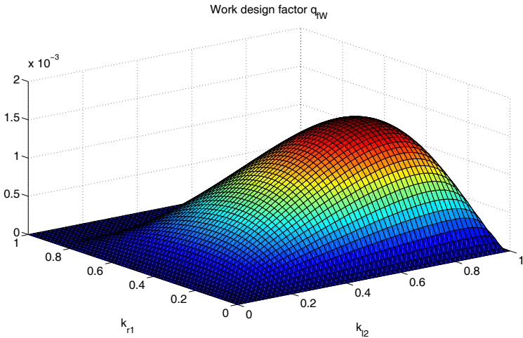
Fig. 3.12 Solenoid work design factor depending on k_{r2} and k_{r1} with \eta = 1.01 and k_{r1} = 0.39
