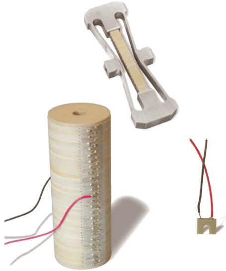
Fig. 1.9 Sample piezoelectric actuators. Courtesy of Noliac
