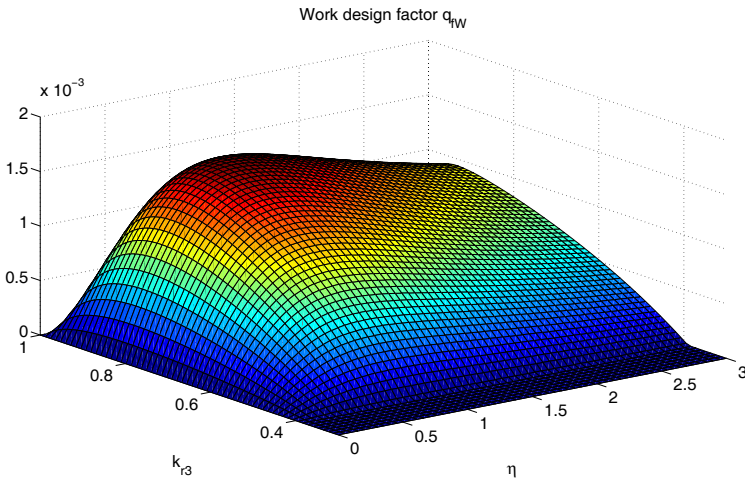
Fig. 3.11 Solenoid work design factor depending on \eta and k_{r3} with k_{r2} = 0.75 and k_{r1} = 0.39
