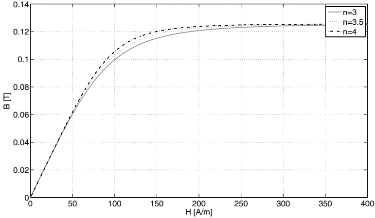
Fig. 2.20 BH saturation curve of Example 2.7
