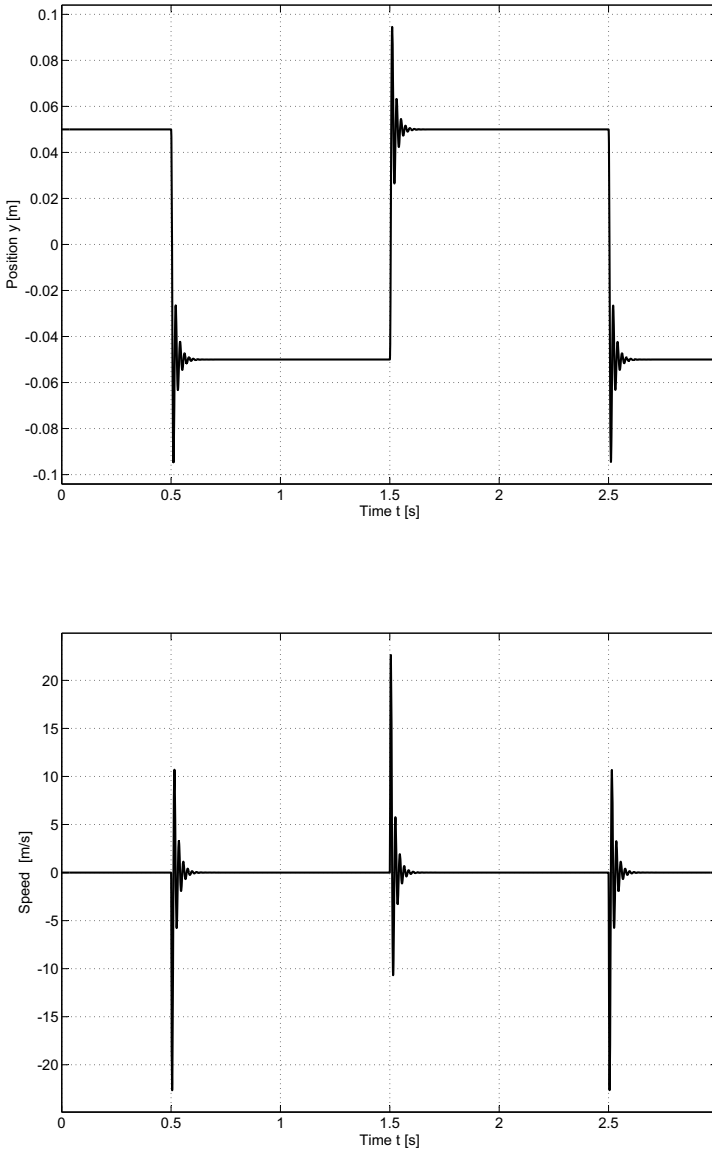
Fig. 5.14 Position and speed response of the hydraulic actuator to an open loop simulation. Simulation 2
