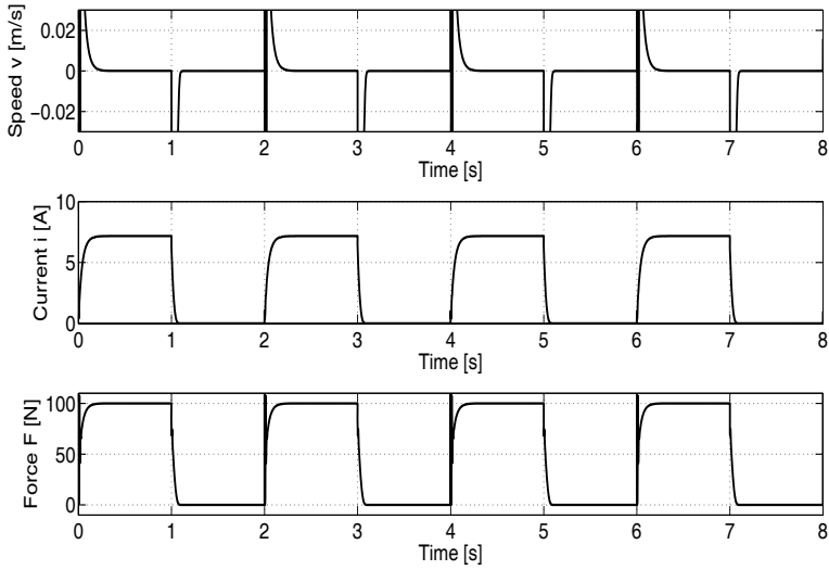
Fig. 3.27 Speed, current and force of the solenoid actuator tracking a rectangular reference
